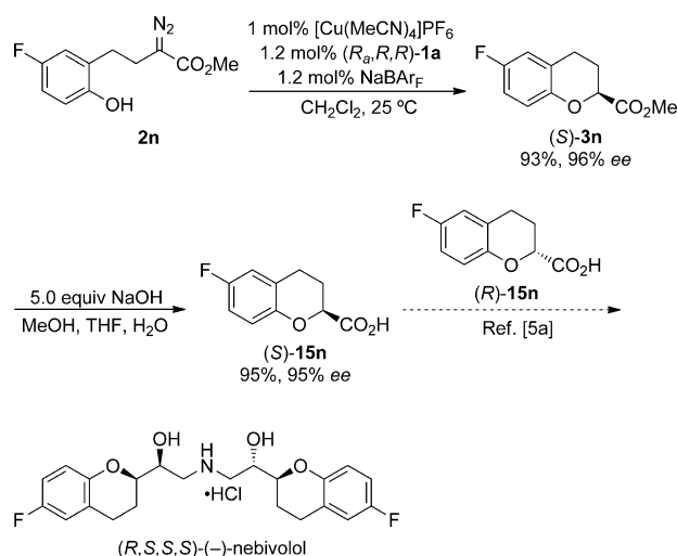
Scheme 2. Formal synthesis of ( R,S,S,S )-(-)-neбиволol.
